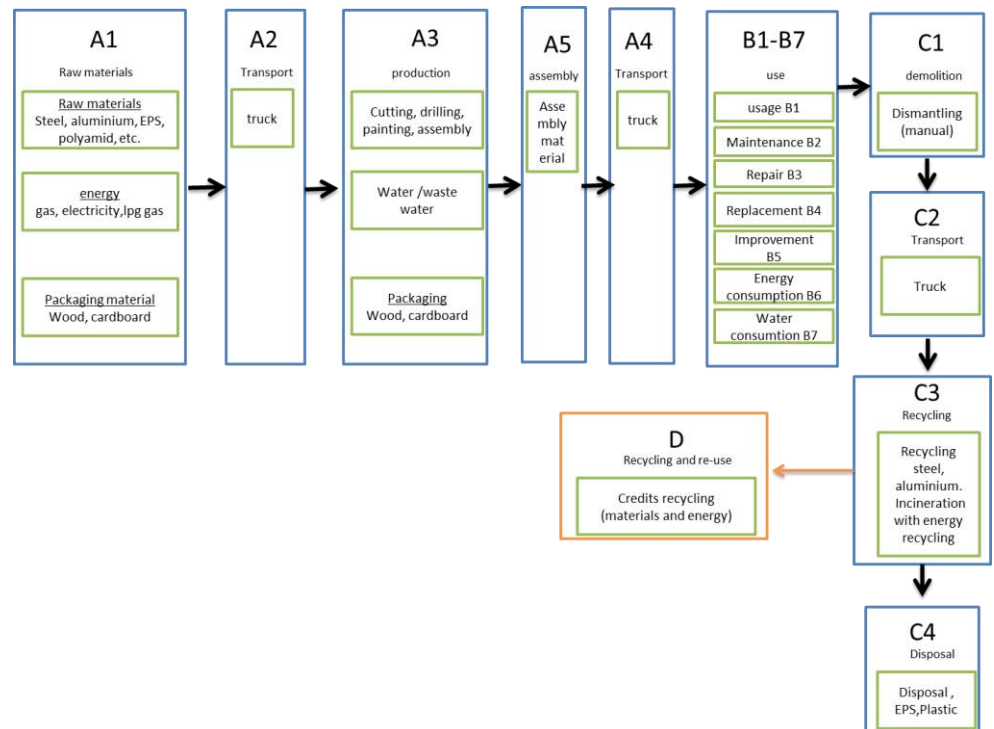
figure 1: Life cycle of the sectional doors
